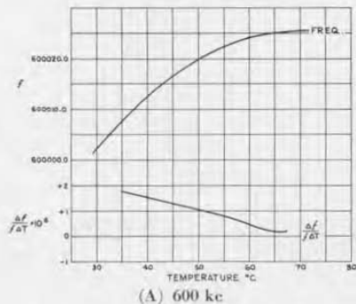
FIGURE 3. Curves showing the variation of both frequency and temperature coefficient of frequency as the temperature is varied for three plates in the standard broadcast band. The upper curves show the change of frequency in cycles per second; the lower curves, the temperature coefficient in parts per million per degree Centigrade
