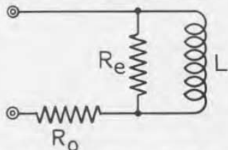
FIGURE 1. Equivalent circuit of a low-frequency coil
